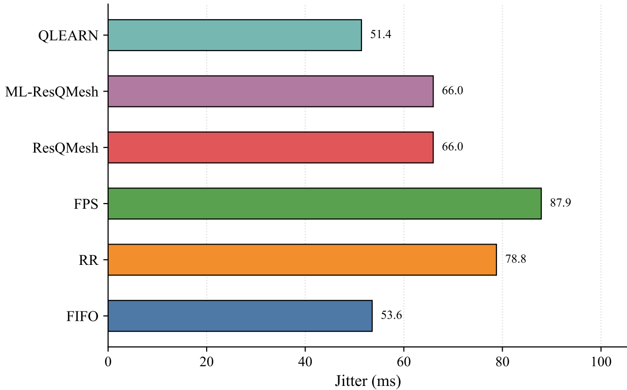
Jitter - Packet Loss
